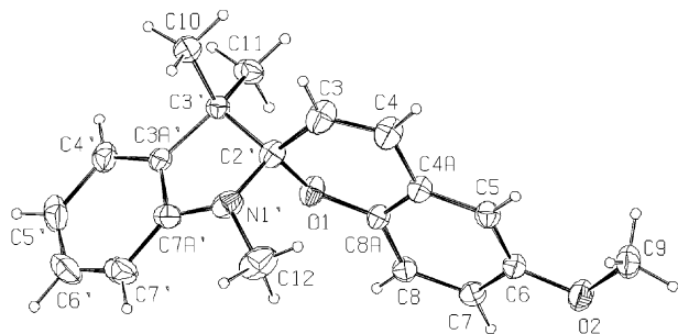
Figure 3. The molecular structure and atom labelling of the indolinospirobenzopyran 9 . Displacement ellipsoid are drawn at the 30% probability level.
