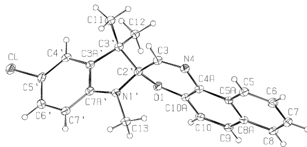
Figure 4. The molecular structure and atom labelling of the indolinospironaphtho-1,4-oxazine 17 . Displacement ellipsoid are drawn at the 30% probability level.
