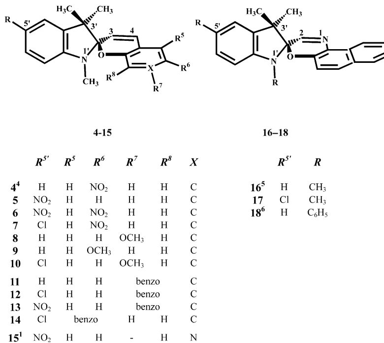
Figure 2. Indolinospirobenzopyrans 4–10 , indolinospironaphthopyrans 11–14 , indolinospiropyridopyran 15 and indolinospironaphtho-1,4-oxazines 16–18 .
