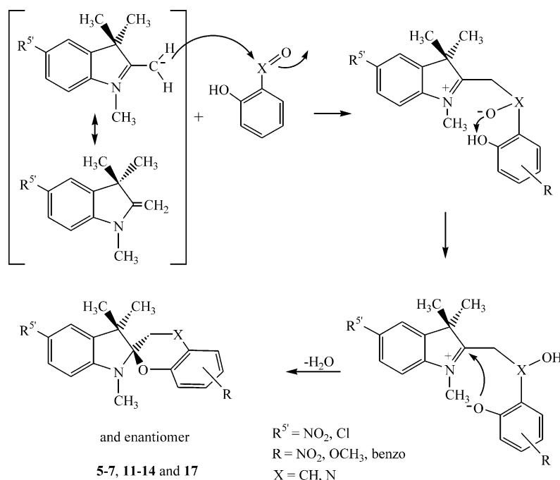
Scheme 1. Synthesis of indolinospirobenzopyrans 5–7 , indolinospironaphthopyrans 11–14 and indolinospironaphtho-1,4-oxazine 17 (c.f. Figs 1 and 2).
